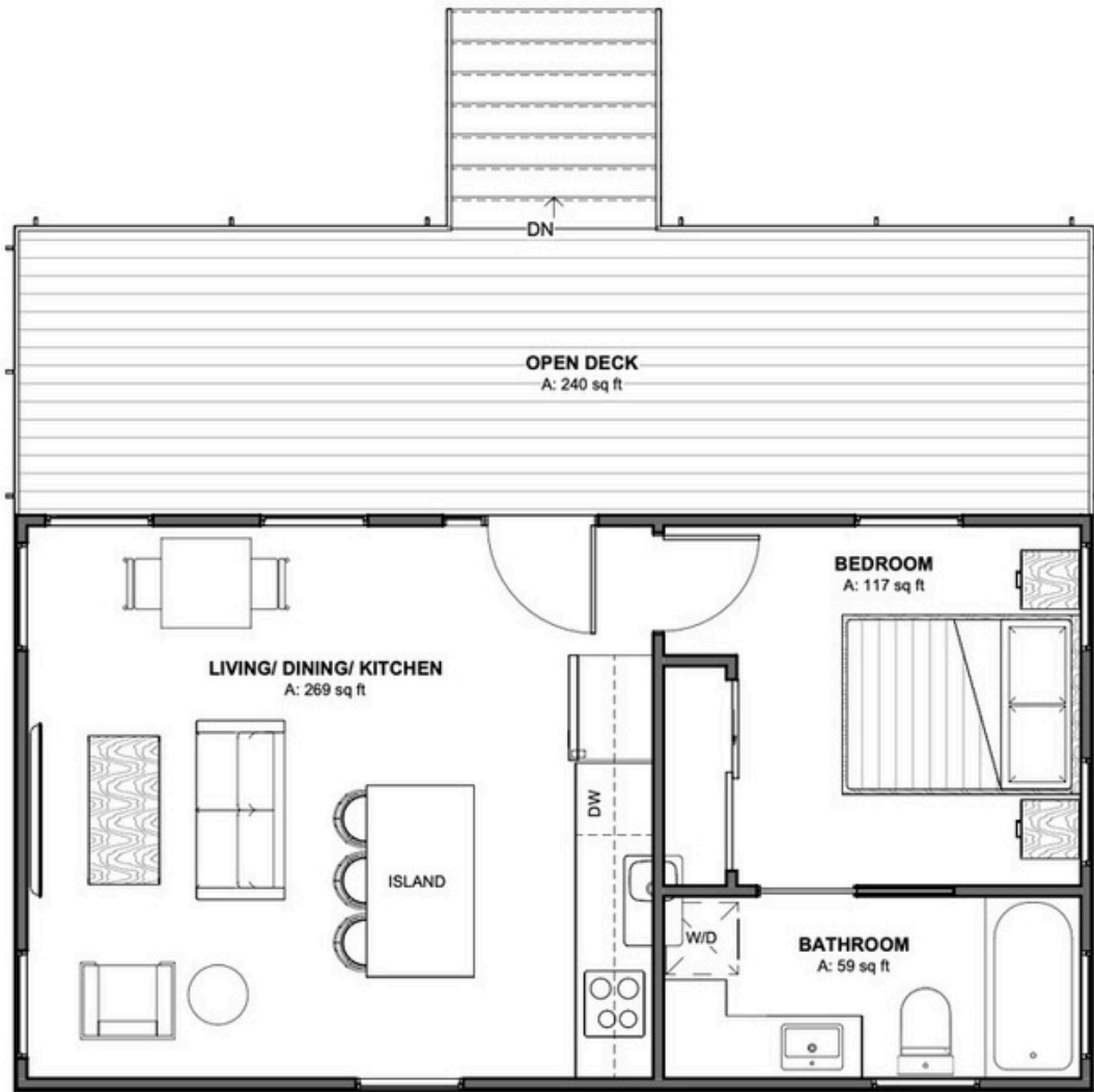
① 1st FLOOR PLAN
