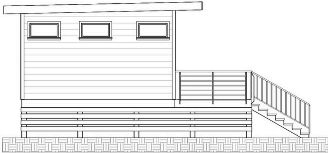
① EAST ELEVATION
