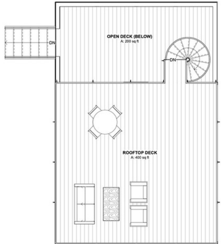
2 ROOF DECK PLAN
