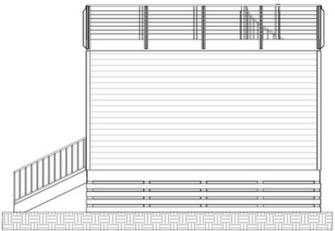
① SOUTH ELEVATION
