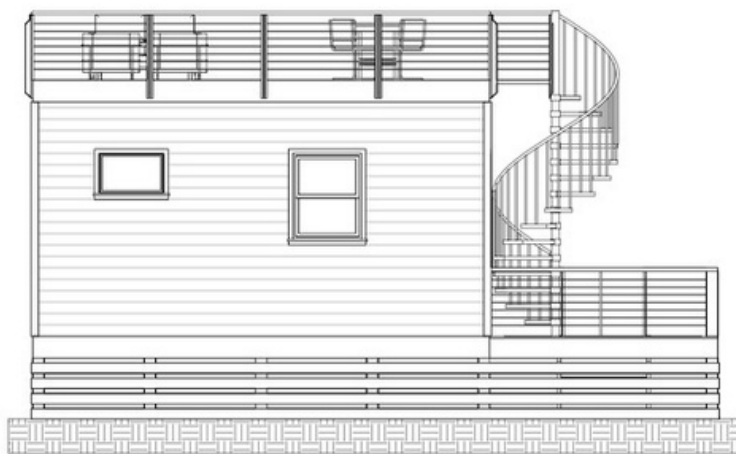
② EAST ELEVATION
