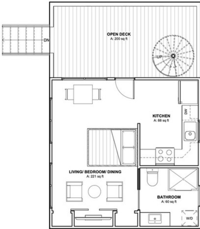
1 1st FLOOR PLAN
