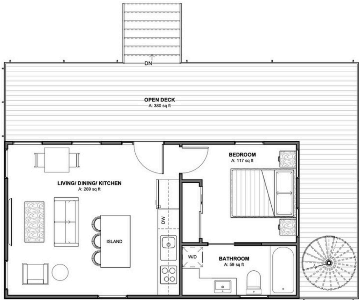
1 1st FLOOR PLAN
