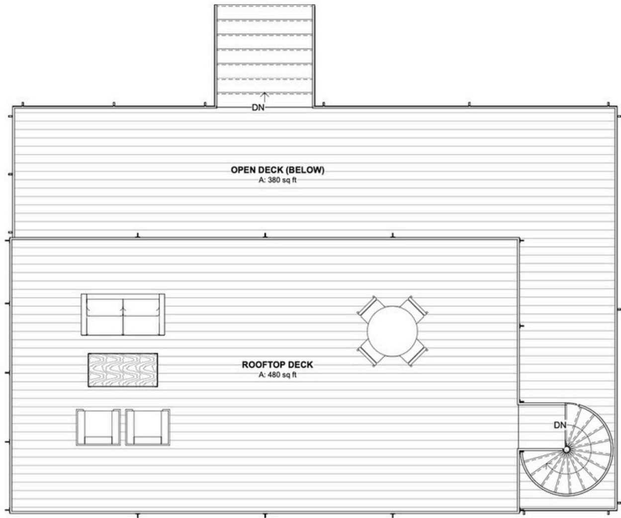
① ROOF DECK PLAN
