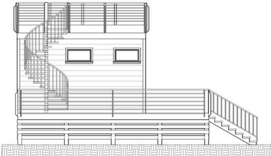
① EAST ELEVATION
