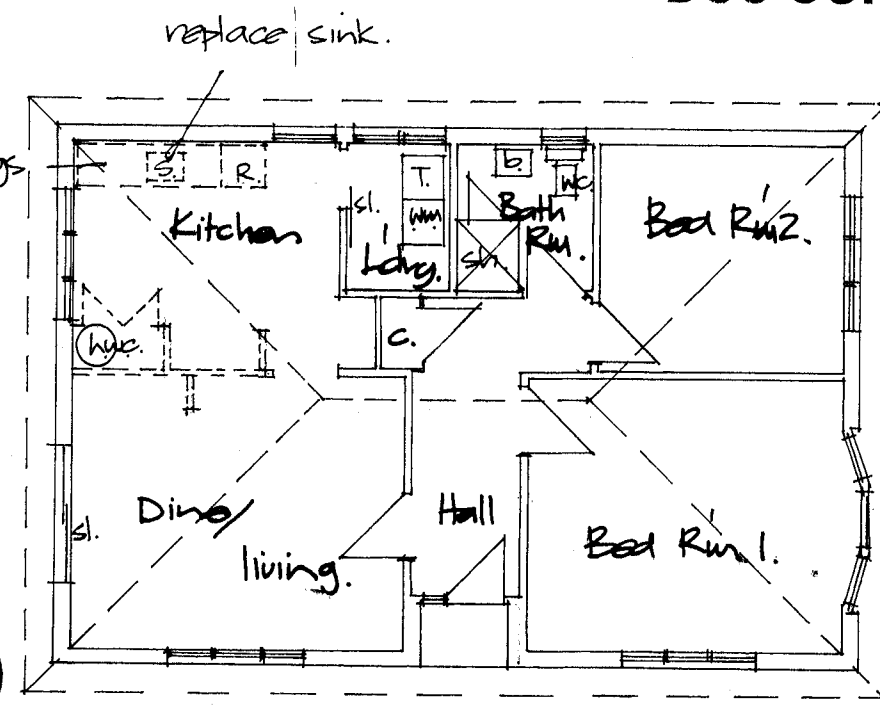
EXISTING FLOOR PLAN 1:100 - showing removal.
