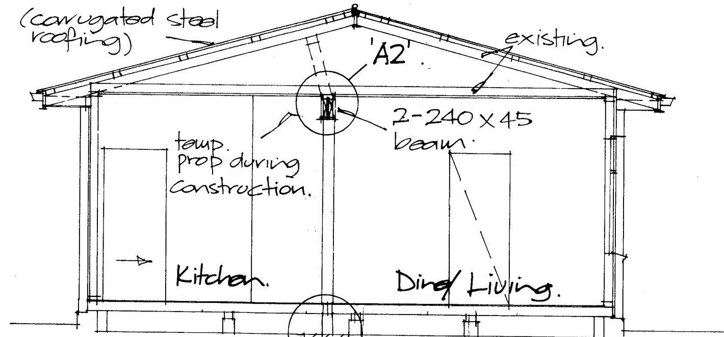
CROSS SECTION 'A-A' 1:50
