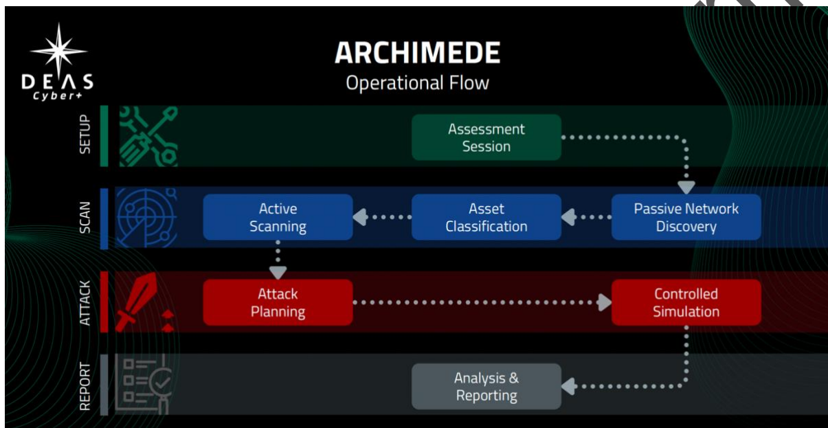
Figure 5: Archimede operational flow.
