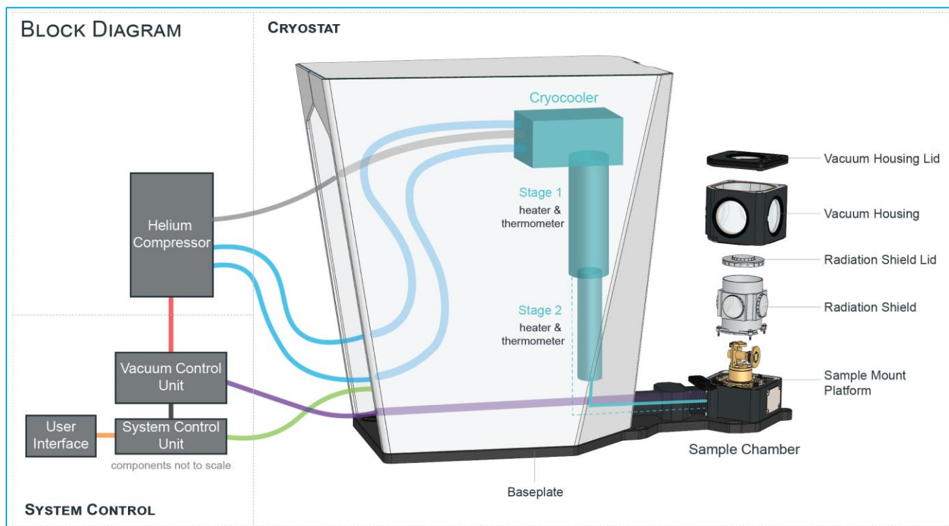
Figure 3: Cryostation connections overview
