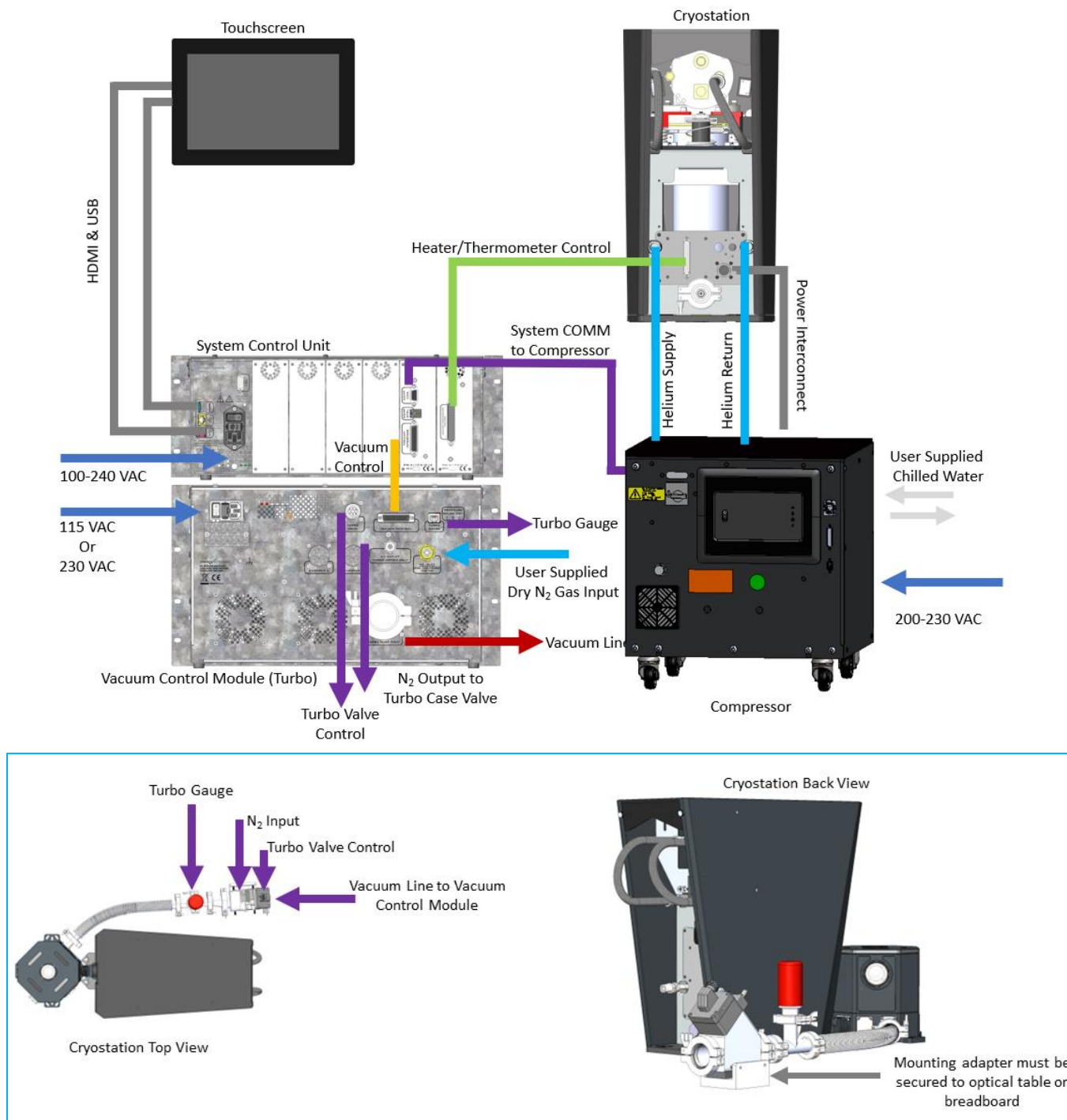
Figure 4*: Cryostation interconnect diagram – Turbo Vacuum Control Module Option
