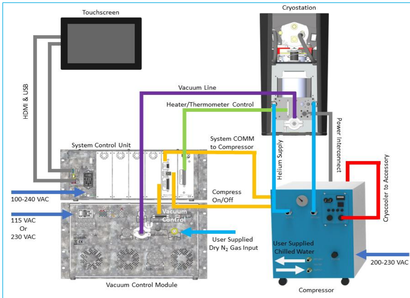
Figure 2: Cryostation system layout, SHI Compressor
