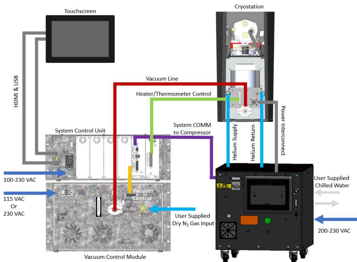
Figure 3*: Cryostation interconnect diagram
