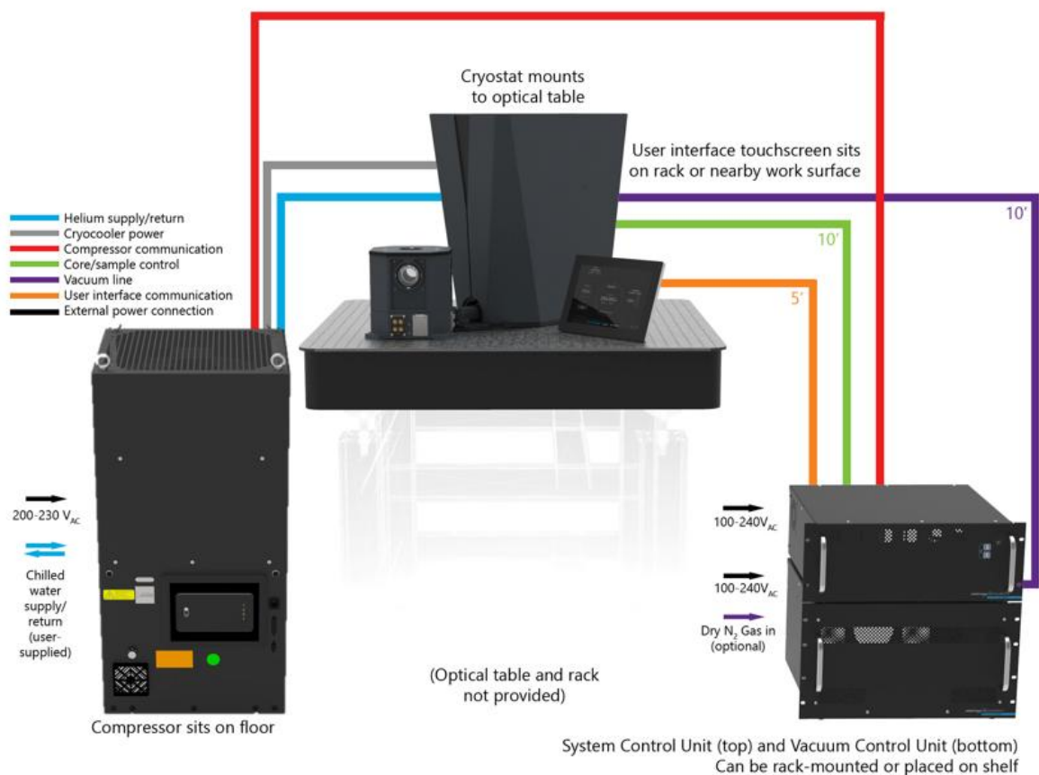
Figure 1: Cryostation system layout, Leybold Compressor
