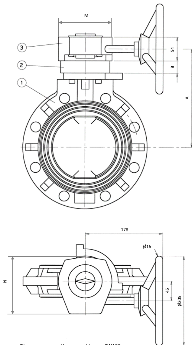
Diagram representing assembly on a DN100
