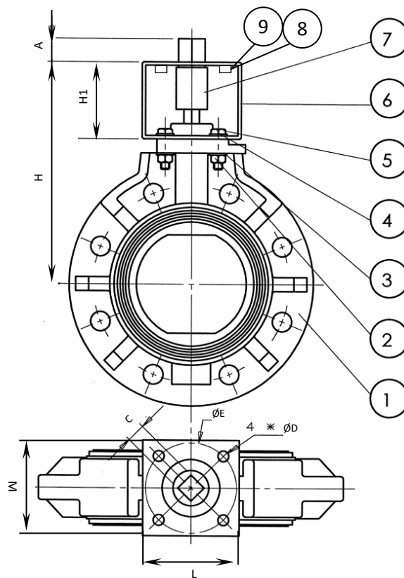
Diagram representing assembly on a DN100
