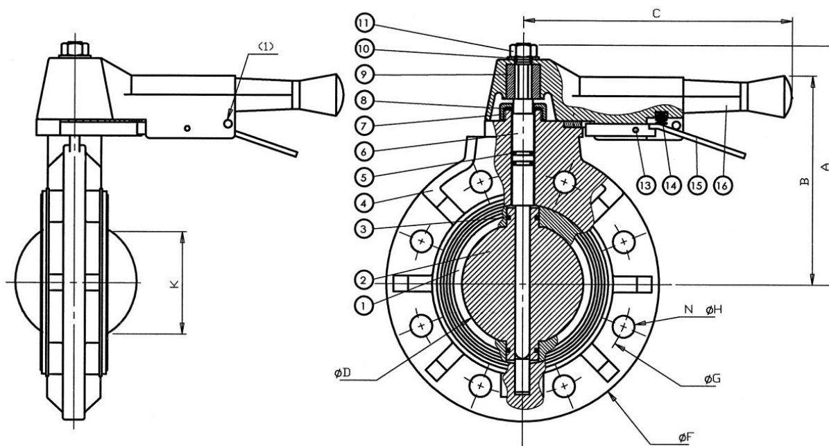
Diagram representing a DN100
