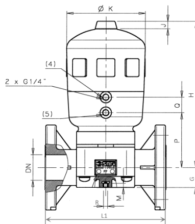
Flanged version
