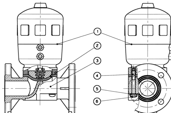
Flanged version
