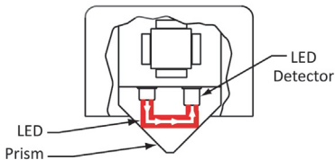
Dry Condition
