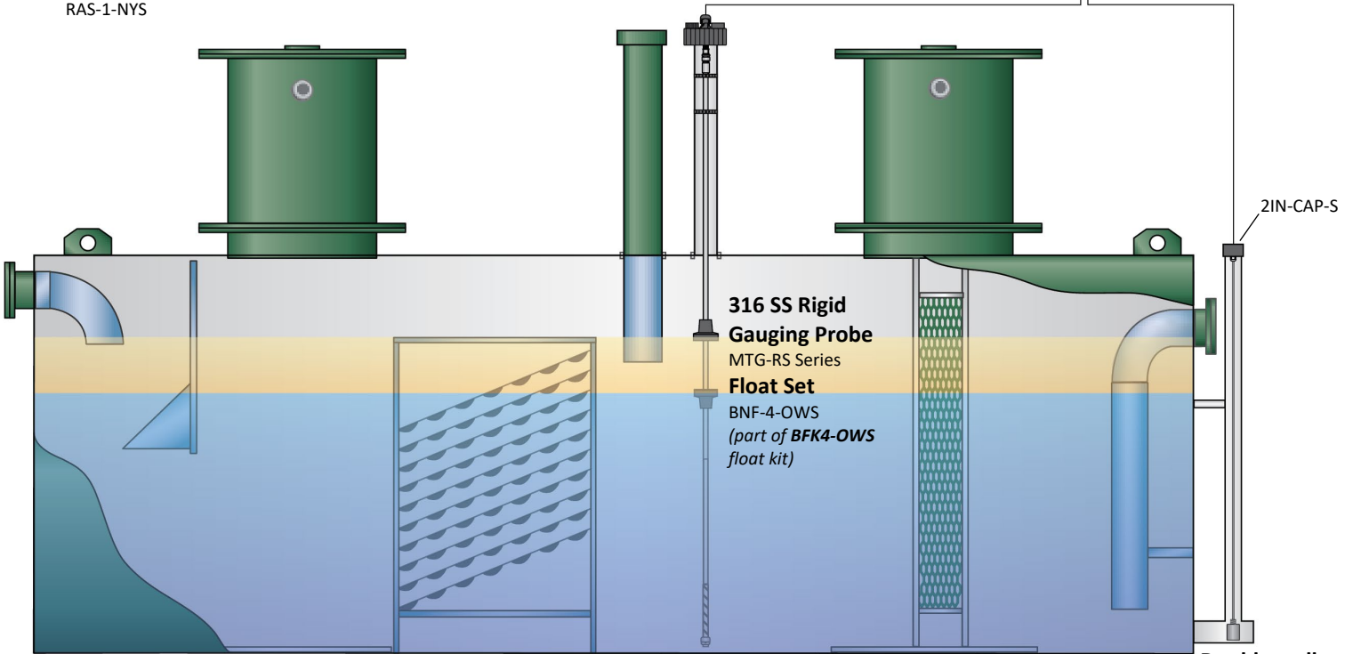
Double wall BX-LWS or BX-PDWS
