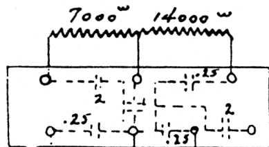
Condenser Block
