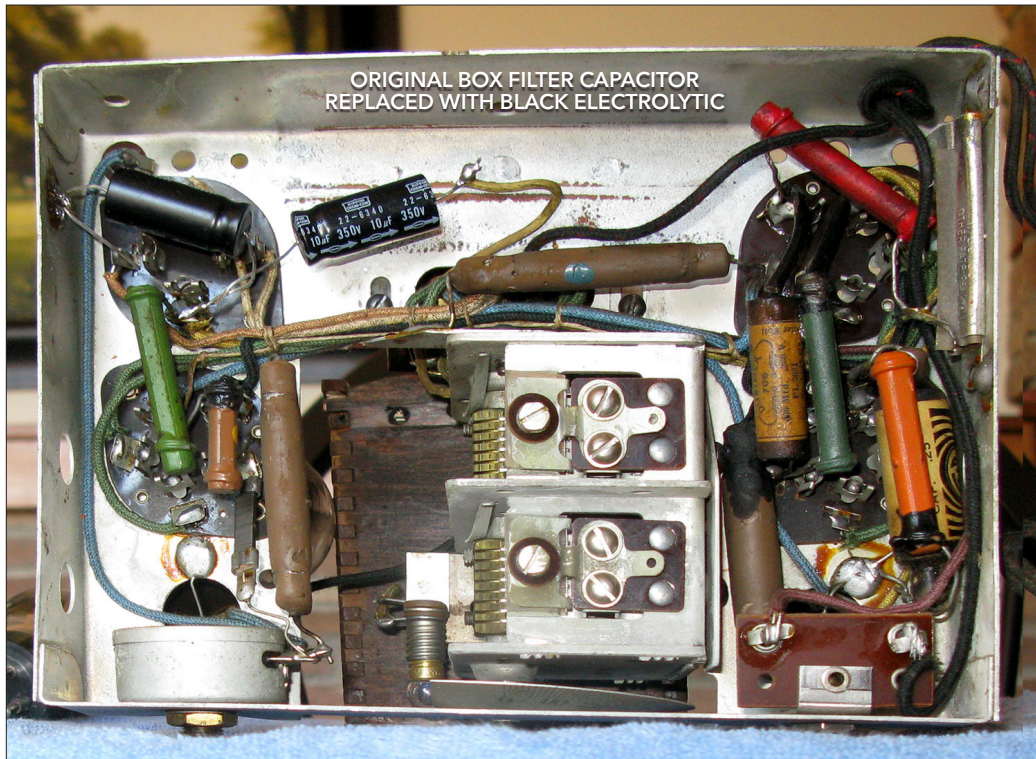
Chassis Bottom View with wooden box support in background Owner provided image (cropped)
