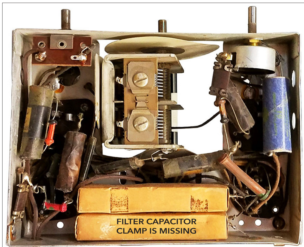
Jackson-Bell Model 84 Willard Cabinet Bottom View
