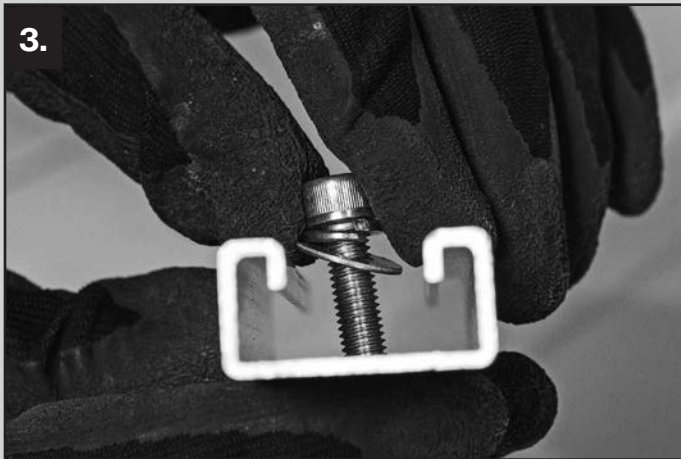
3. Assemble the 8 mm bolt, lock washer and washer and put through the pre-drilled hole in the mounting track.
