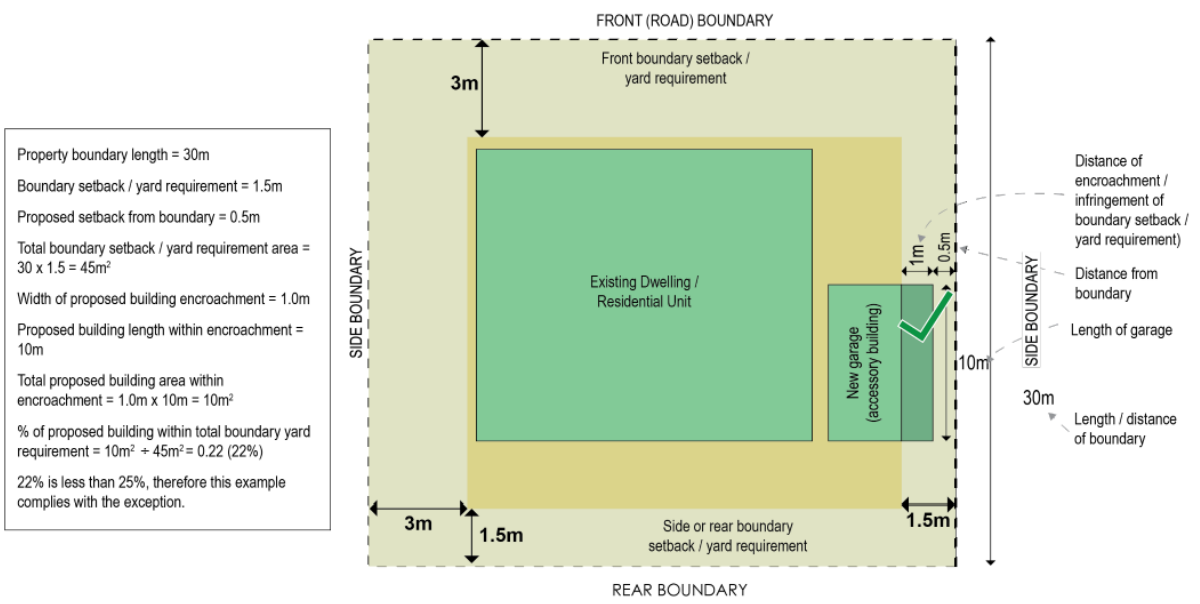
GRZ Diagram 2: Setback exemptions for accessory buildings
