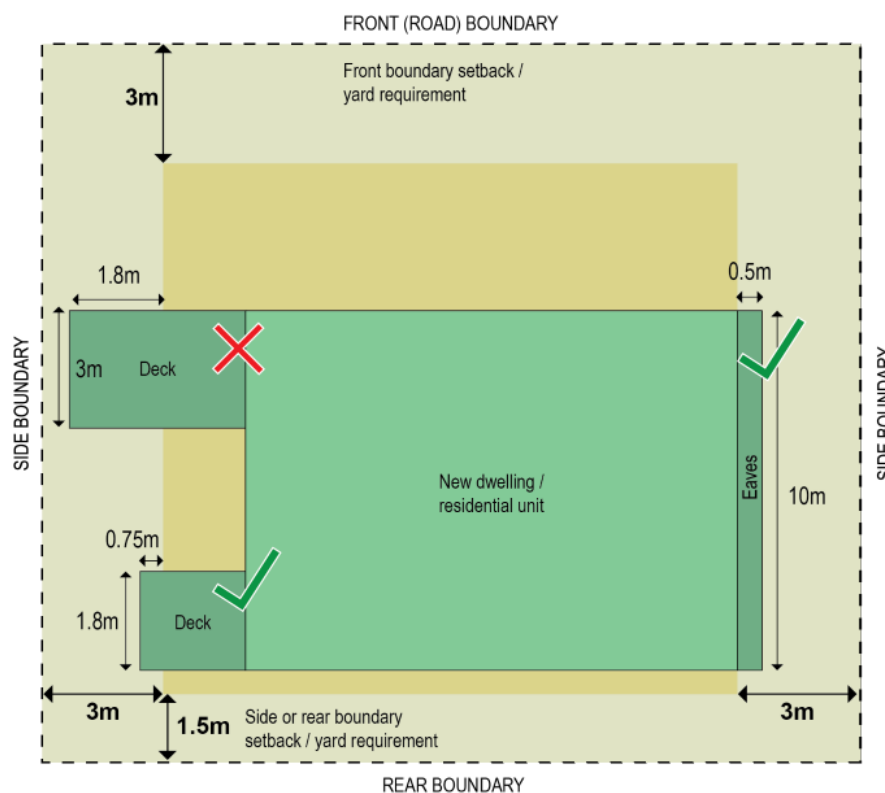
GRZ Diagram 1: Setback exemptions for eaves, porches, balconies, decks, and other minor building features
