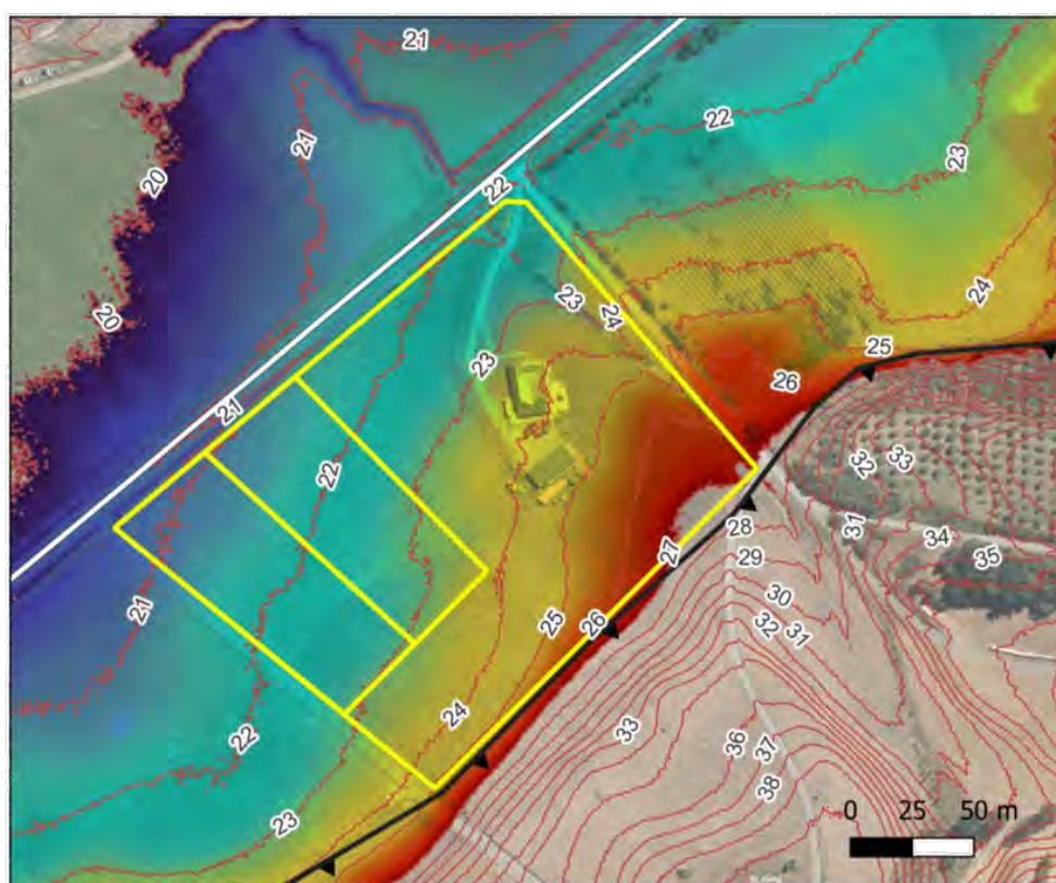
Figure 7 Topographic map for site and adjacent areas, 1m contours and colour overlay derived from LiDAR data. The mapped backthrust fault is as per Figure 6.
