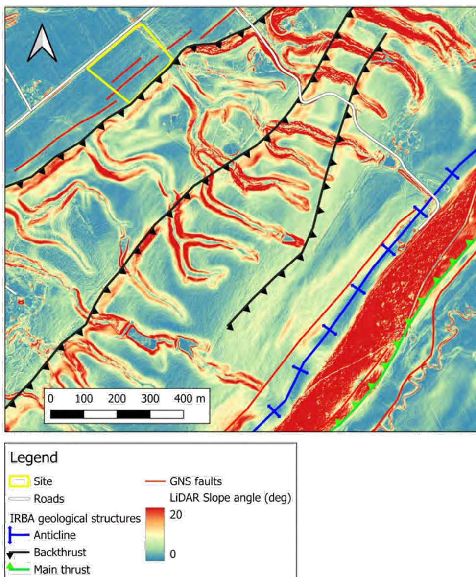
Figure 6 Geological interpretation for central Te Maire fault zone, overlain over LiDAR slope angle map. Main thrust location taken from GNS.
