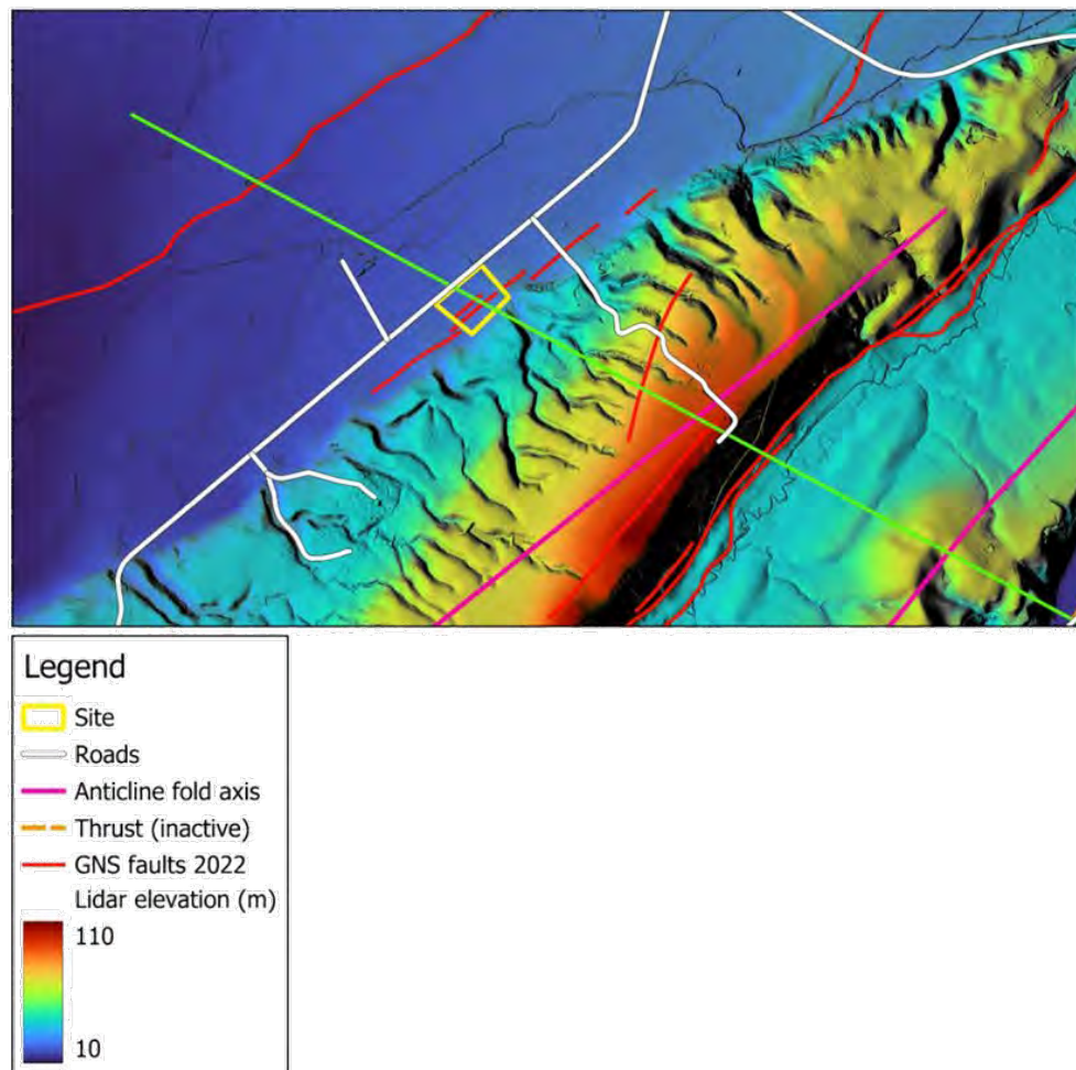
Figure 2 LIDAR topographic map across central Te Maire Fault.
