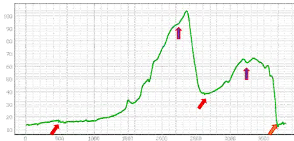
Figure 3 NW to SE cross section through Bidwill Hill ridge. Active thrust faults indicated with red arrows, inactive thrust fault indicated with orange arrow. Purple arrows indicate axes of anticline (upwards) folds. Cross section location shown on Figure 2. Vertical exaggeration 15:1
