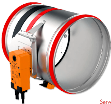
Servomotor
