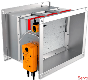
Servomotor
