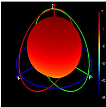
Phi=90 freq=1227MHz
