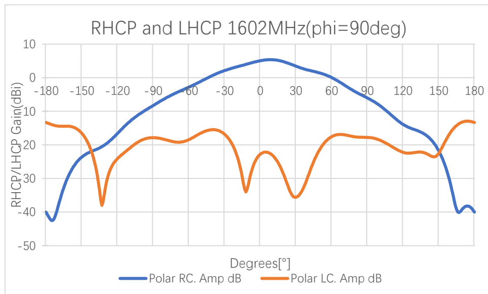
2D RHCP and LHCP Gain (dBi)
