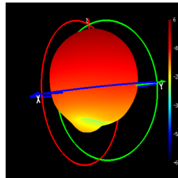
Phi=90 freq=1248MHz
