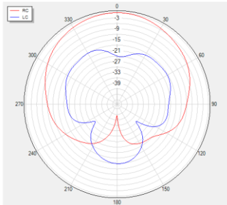
Phi=0 freq=1575MHz
