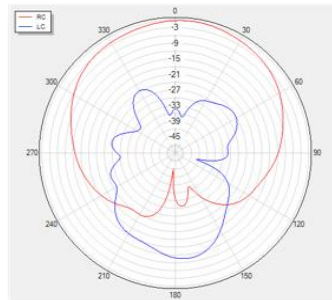
Phi=90 freq=1207MHz
