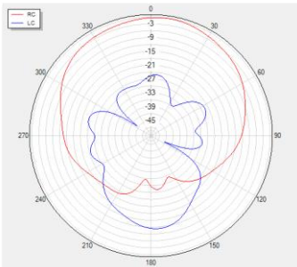
Phi=90 freq=1268MHz
