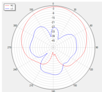
Phi=90 freq=1602MHz
