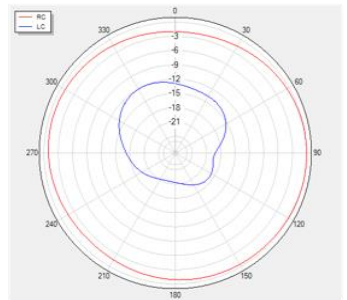
Theta=90 freq=1207MHz
