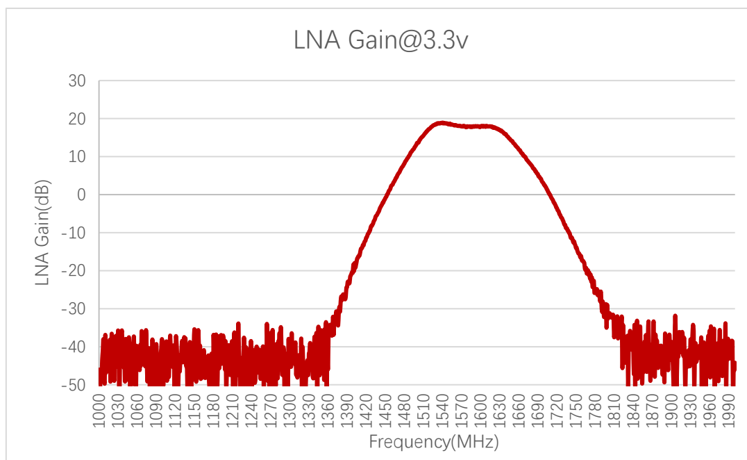
LNA Gain (dB)
