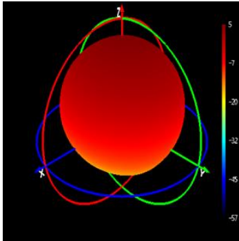
Phi=90 freq=1176MHz
