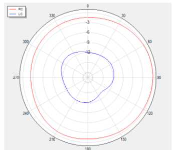
Theta=90 freq=1602MHz
