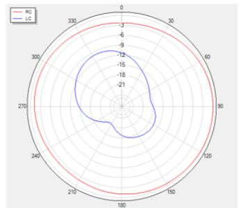
Theta=90 freq=1248MHz
