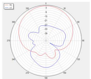
Phi=0 freq=1248MHz
