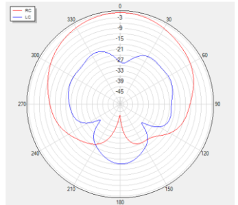
Phi=0 freq=1602MHz
