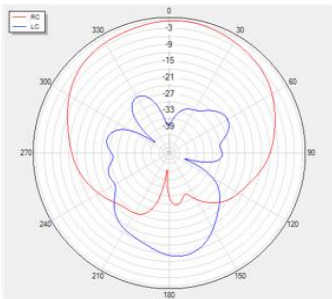
Phi=90 freq=1227MHz
