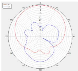
Phi=0 freq=1227MHz
