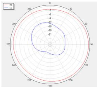
Theta=90 freq=1227MHz
