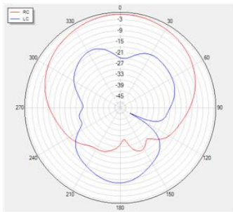
Phi=0 freq=1176MHz
