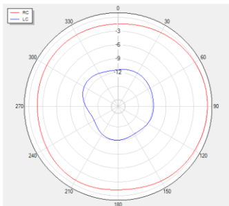
Theta=90 freq=1575MHz
