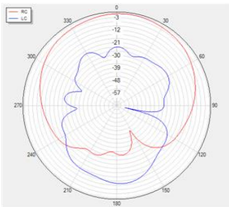
Phi=90 freq=1176MHz
