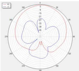
Phi=90 freq=1575MHz
