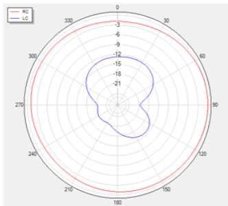
Theta=90 freq=1176MHz
