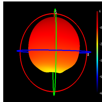
Phi=90 freq=1602MHz
