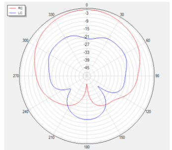
Phi=0 freq=1561MHz
