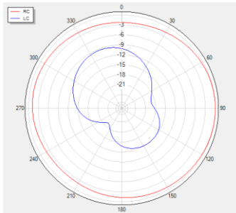
Theta=90 freq=1268MHz
