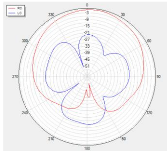
Phi=90 freq=1561MHz
