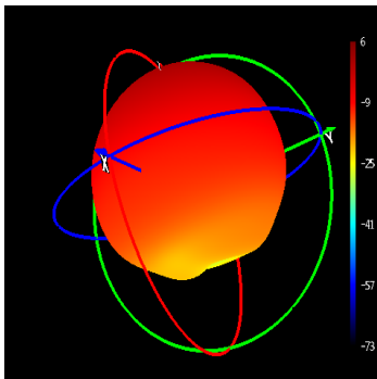
Phi=90 freq=1575MHz
