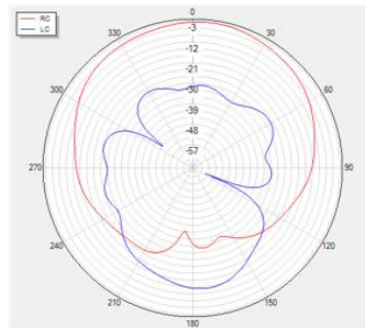
Phi=90 freq=1248MHz
