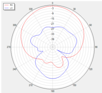
Phi=0 freq=1268MHz
