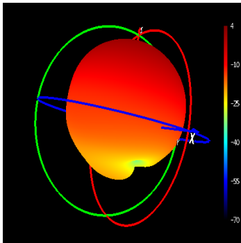
Phi=90 freq=1268MHz
