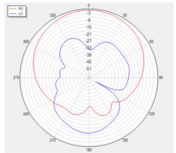
Phi=0 freq=1207MHz
