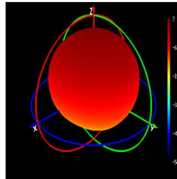
Phi=90 freq=1561MHz
