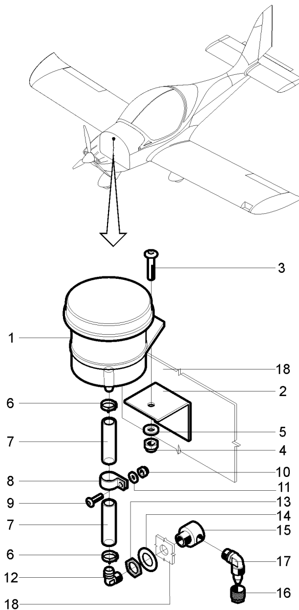
Fig.2, page 1 Removal of the hydraulic fluid reservoir
