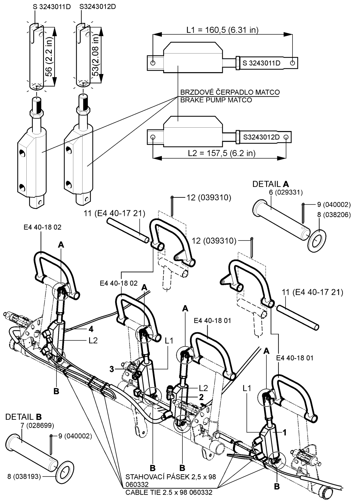
Fig. 4 Installation of brake pumps
