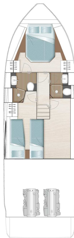
LOWER DECK
