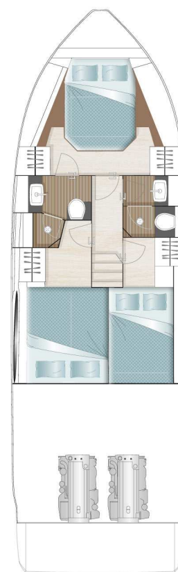
LOWER DECK
