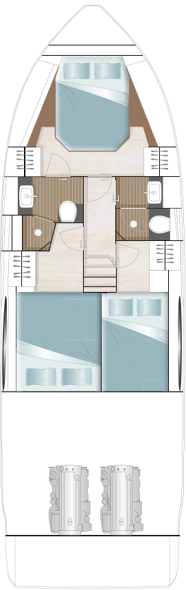
LOWER DECK Portside cabin with queen-size double bed, starboard cabin with double bed option
