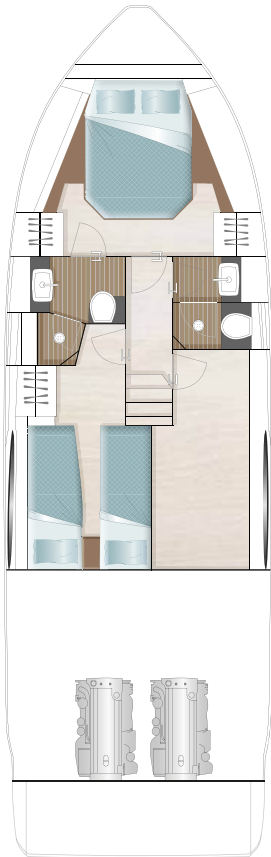
LOWER DECK Portside double cabin with two single berths, starboard storage room standard
