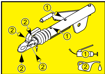
Fig. 1: Lubrication points on the coupling
