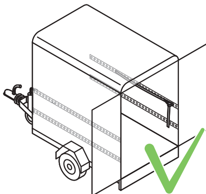
Fig. 31: Correctly lashed load
