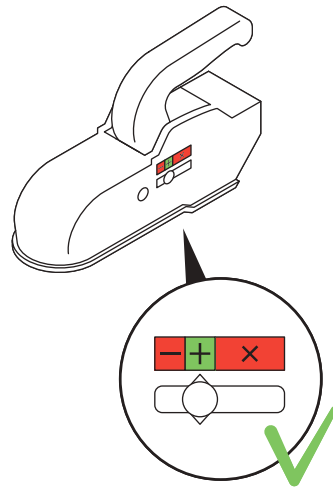
Fig. 6: Safety and wear indicator for coupling A1
