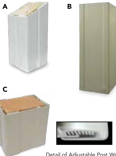
Detail of Adjustable Post Wrap Ratcheting System Adjustable in 0.125" Increments
