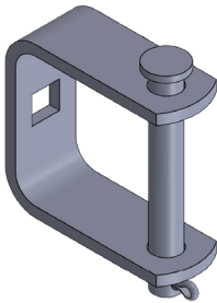
Insulated Deadend Clevis C-3325
