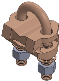
Bronze U-Bolt Ground Clamp UGC-2
