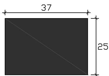
Art. SCS-285-TS Des.SETTING BLOCK Mtl. SCR-TS Hs. 85° Ref. 531,
