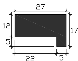
Art. SCS-290-TS Des.SETTING BLOCK Mtl. SCR-TS Hs. 85° Ref. B3A846A,768,
