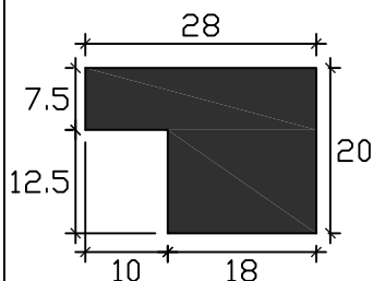
Art. SCS-283-TS Des.SETTING BLOCK Mtl. SCR-TS Hs. 85° Ref. GK-06,456,
