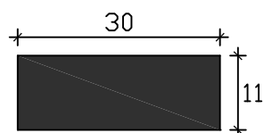
Art. SCS-294-TS Des.SETTING BLOCK Mtl. SCR-TS Hs. 85° Ref. GK-16,EPS-091,
