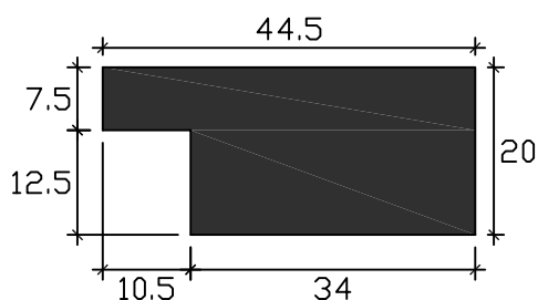
Art. SCS-282-TS Des.SETTING BLOCK Mtl. SCR-TS Hs. 85° Ref. GK-05,456,
