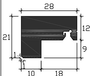
Art. SCS-288-TS Des.SETTING BLOCK Mtl. SCR-TS Hs. 85° Ref. B1C96A,768,
