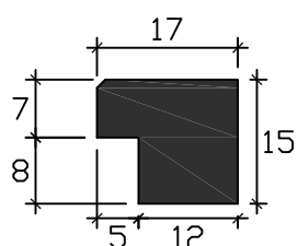
Art. SCS-289-TS Des.SETTING BLOCK Mtl. SCR-TS Hs. 85° Ref. BBK017A,768,
