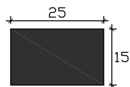
Art. SCS-287-TS Des.SETTING BLOCK Mtl. SCR-TS Hs. 85° Ref. B3A826A,768,
