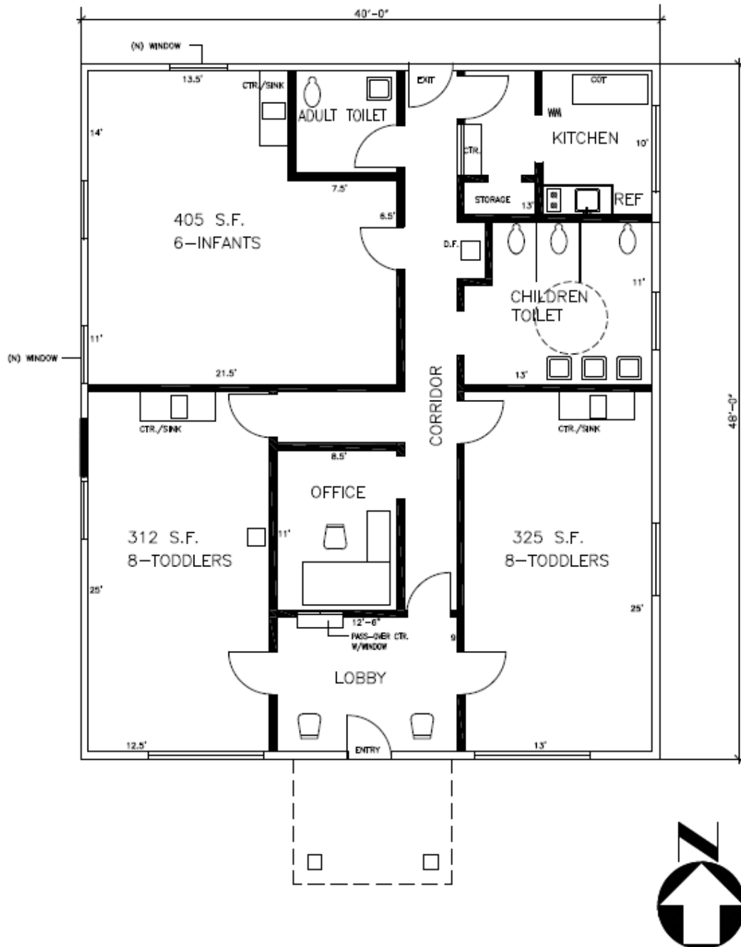
PROPOSED CLASSROOMS FLOOR PLAN SCHEME "C"
