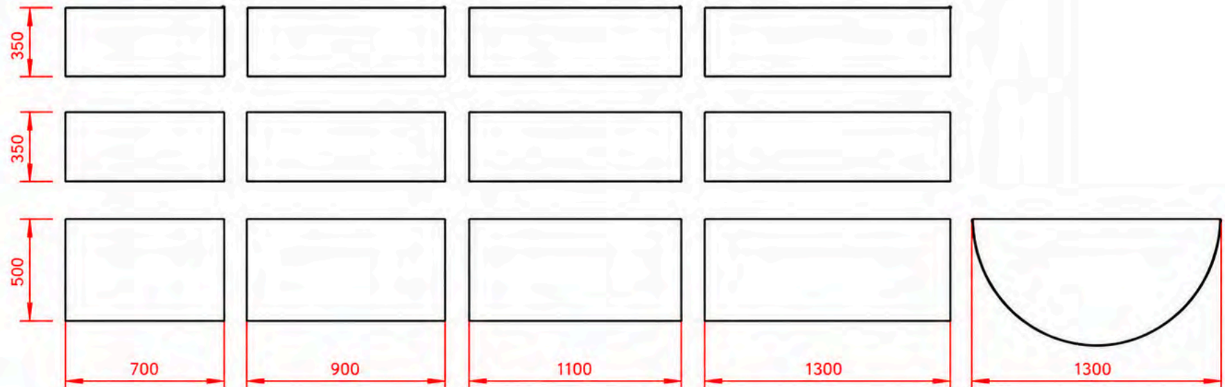
Top view
