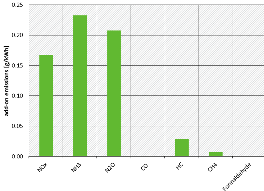
Figure 25: Add-on emissions from 50 000 km to 700 000 km for an average German traffic situation, long haul trucks, Euro VI DE 26
