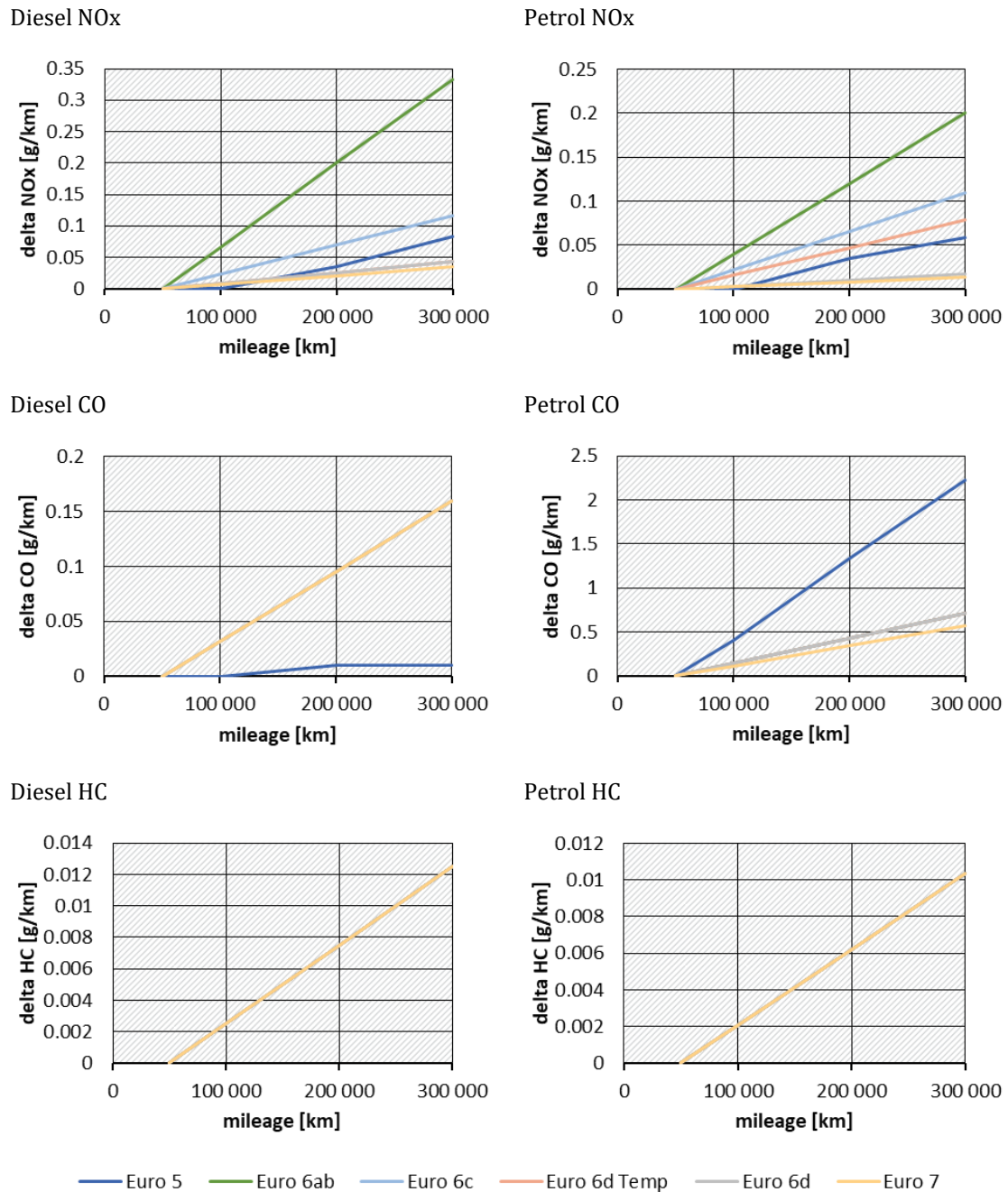
Figure 22: deterioration functions for NO x , CO and HC for petrol and diesel vehicles
