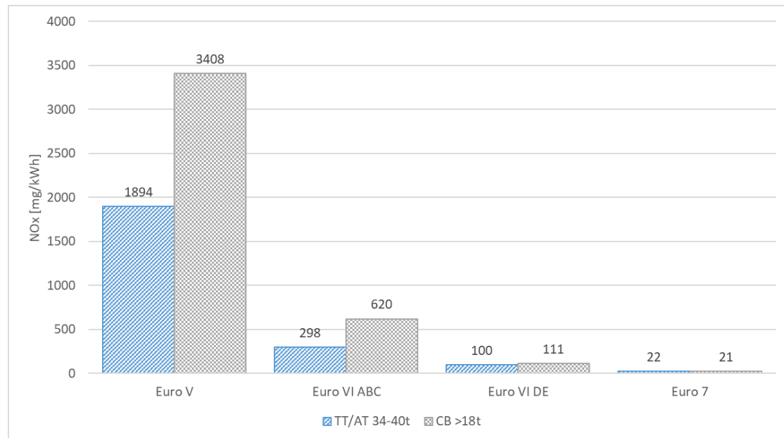
Figure 13: NO x emission factors, tractor trailer combination in German average motorway driving and 3-axis urban bus (or “city bus”, CB) in German average urban driving
