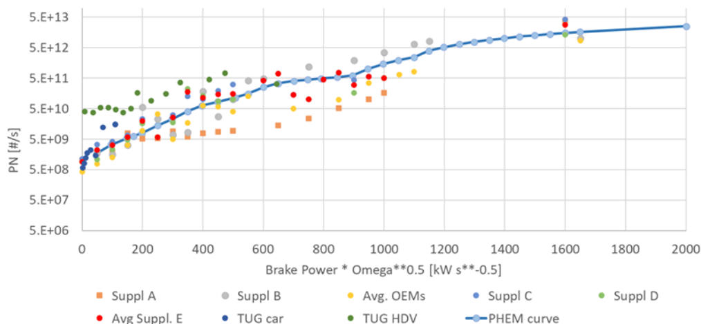
Figure 28: Brake emission polygons for ECE brake systems and average polygon used for all vehicle segments up to EURO 6/VI in this study
