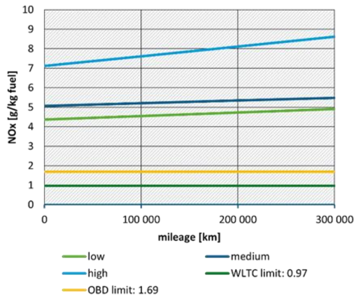
Figure 21: NO x emissions of diesel Euro 6abc cars over vehicle mileage, differentiated by engine load. Source: (Kumawat and Borken-Kleefeld 2025)
