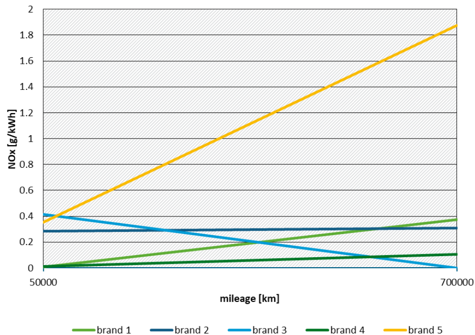
Figure 24: Absolute emissions over mileage per manufacturer, NO x , Euro VI DE, long-haul trucks
