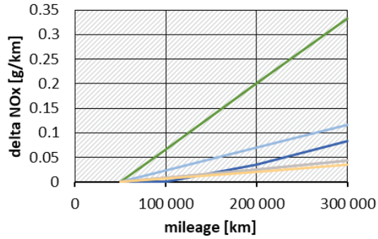
Figure 22: deterioration functions for NO x , CO and HC for petrol and diesel vehicles
