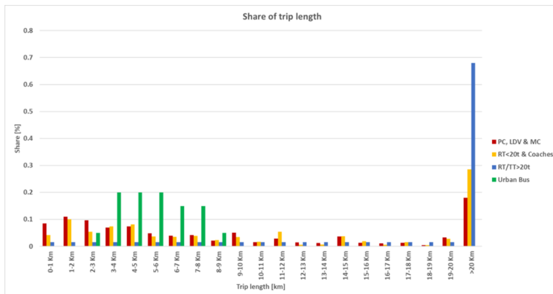
Figure 14: Trip length distributions used for AT in HBEFA 5.1.
