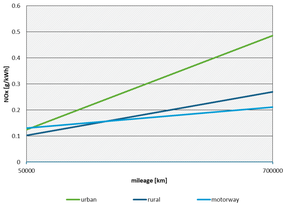
Figure 23: Emissions over mileage per road category, NOx, Euro VI DE, long-haul trucks
