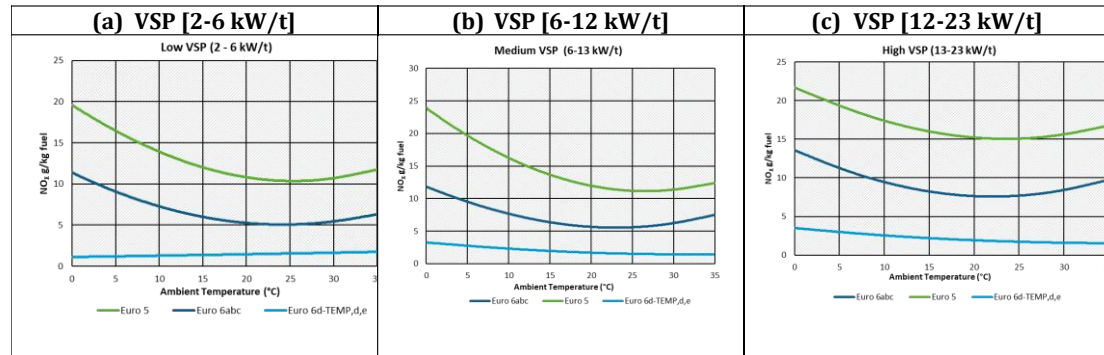
Figure 27: Average NO x emissions as a function of ambient temperature for diesel cars (Euro 5, Euro 6abc, Euro 6d-TEMP,6d, e) modelled using LinearGAM
