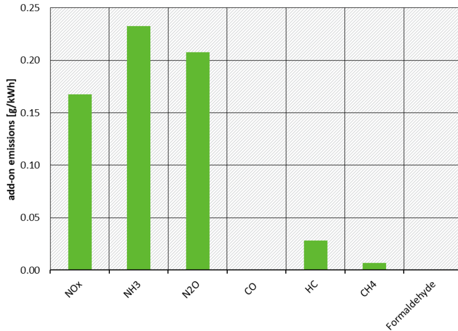
Figure 25: Add-on emissions from 50 000 km to 700 000 km for an average German traffic situation, long haul trucks, Euro VI DE 26
