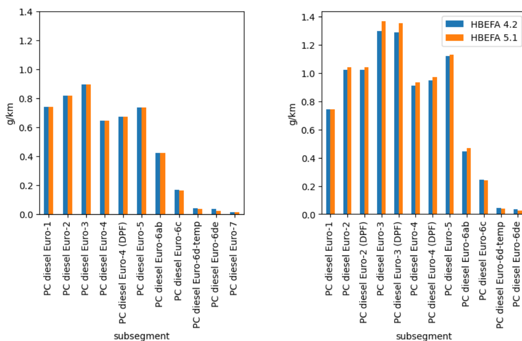
Figure 1: Hot uncorrected (left) and corrected (for year 2025, right) NO x EF of Diesel PC, HBEFA 5.1 vs. 4.2 (Swiss overall aggregate TS).
