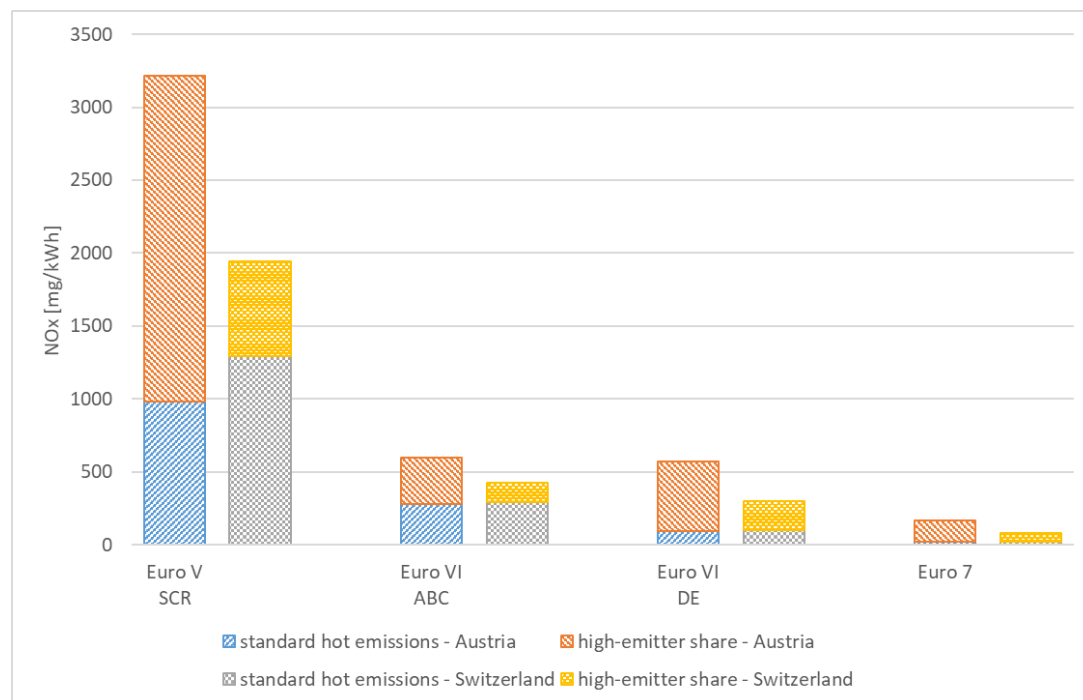
Figure 31: NO x fleet emissions – standard emission factors + high-emitter emissions, tractor trailer combination, average driving
