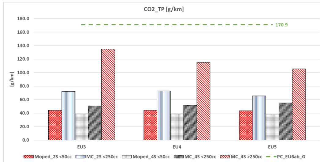
Figure 6: HBEFA 5.1 CO 2 emissions of motorcycles in the German traffic situation mix
