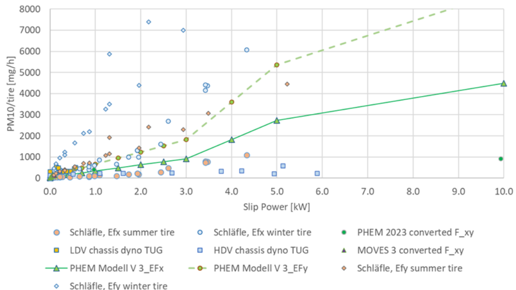
Figure 29: Characteristic tire wear polygons for PM10 emissions due to longitudinal (EF x ) and lateral slip (EF y ) for simulation in PHEM, as well as available measurement and literature data
