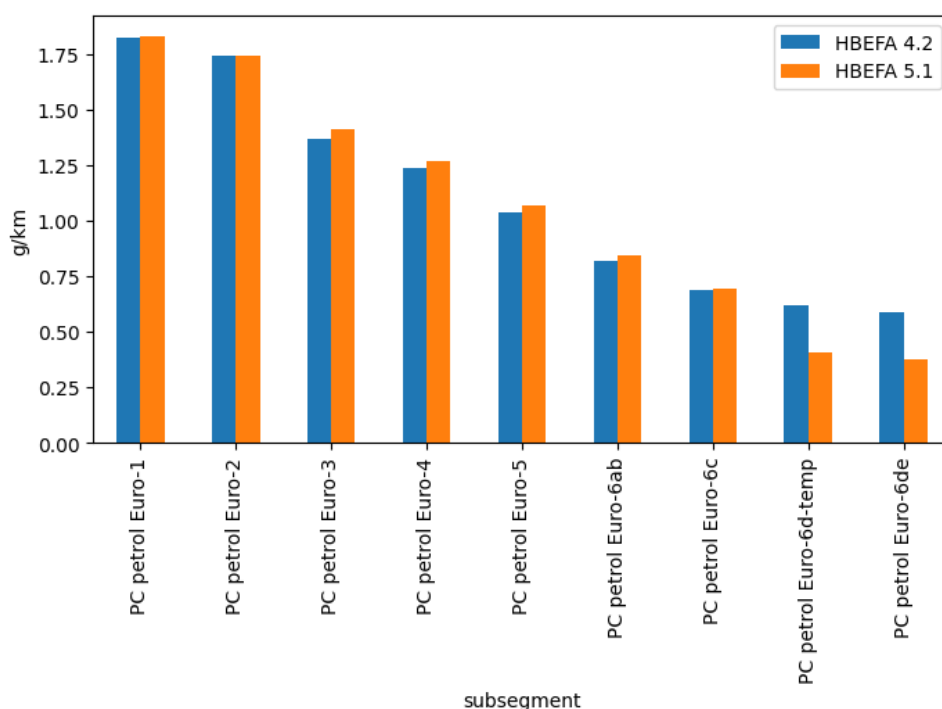
Figure 30: Diurnal evaporation HC emission factors for petrol passenger cars.
