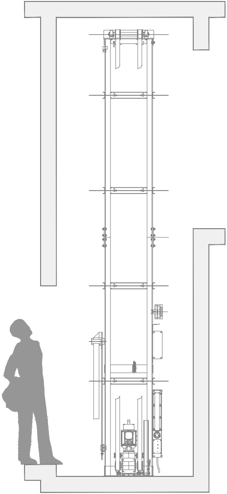
TRACTION DRIVE SYSTEM
