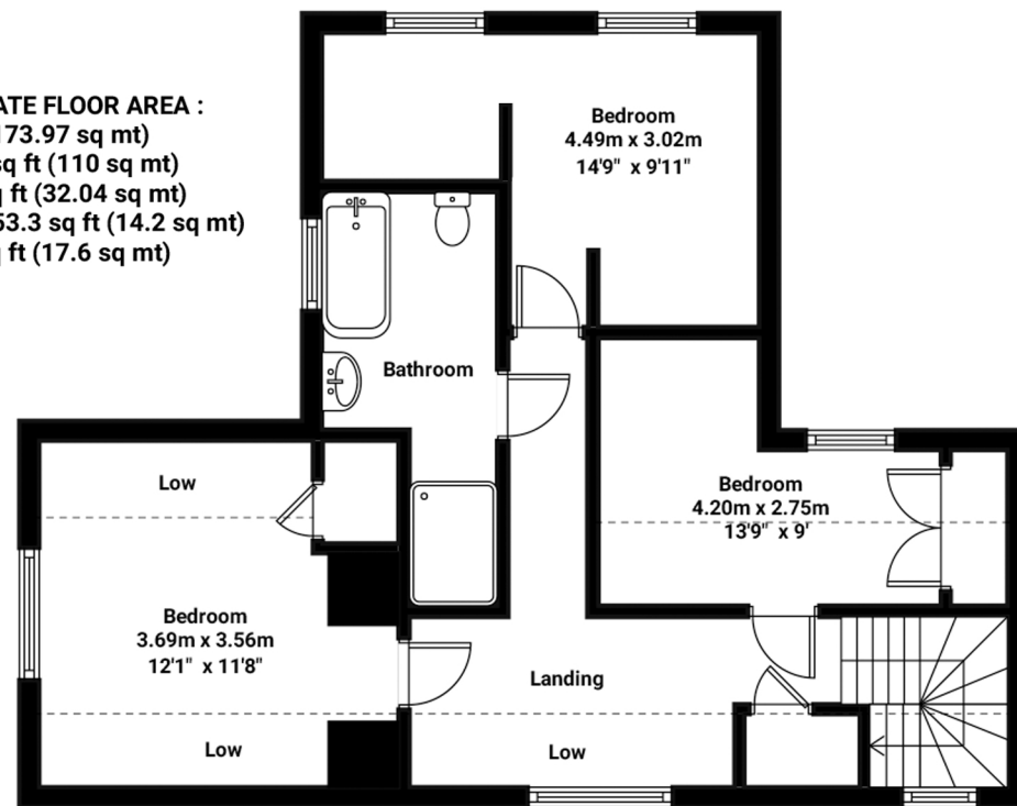
FIRST FLOOR
