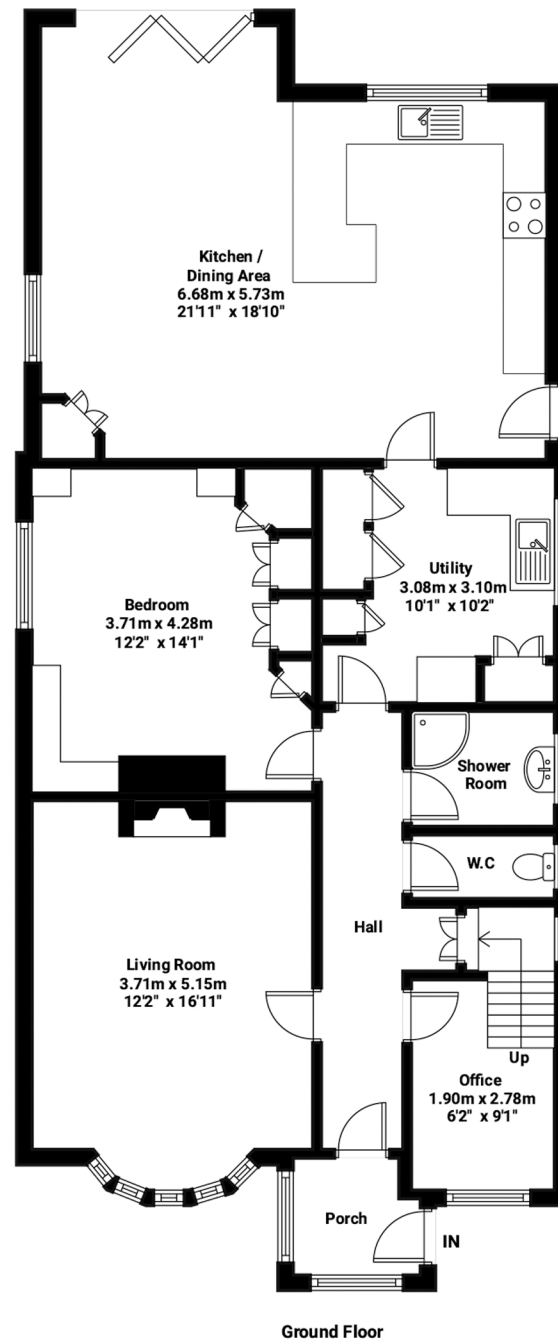
Ground Floor
