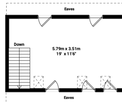
Garage First Floor
