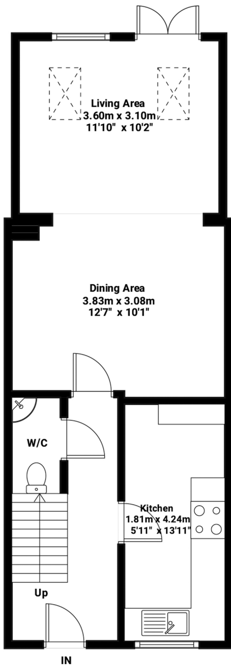
Ground Floor
