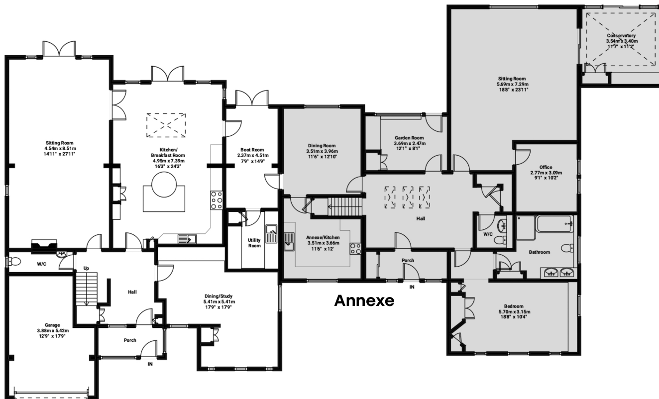
Ground Floor Main House
