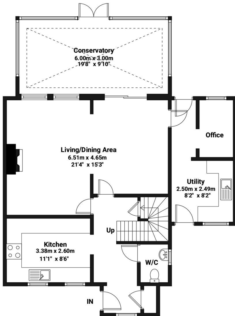
Ground Floor
