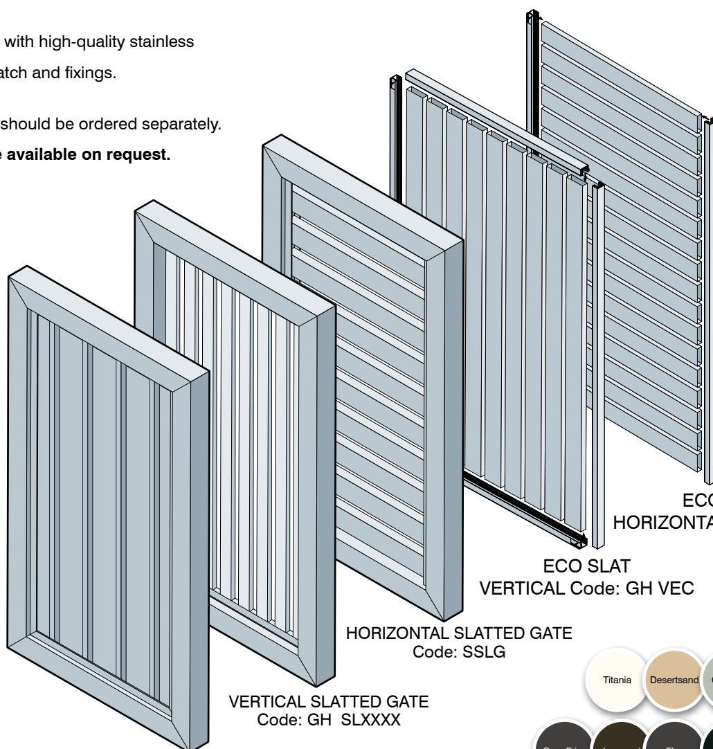
COLOURED STEEL GATE Code: SSHG
