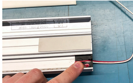
Step 2: Dry fit and mark location for feed location exit. On mounting surface, drill a hole for feed wire to exit. (Min. of 3/4" DIA)
