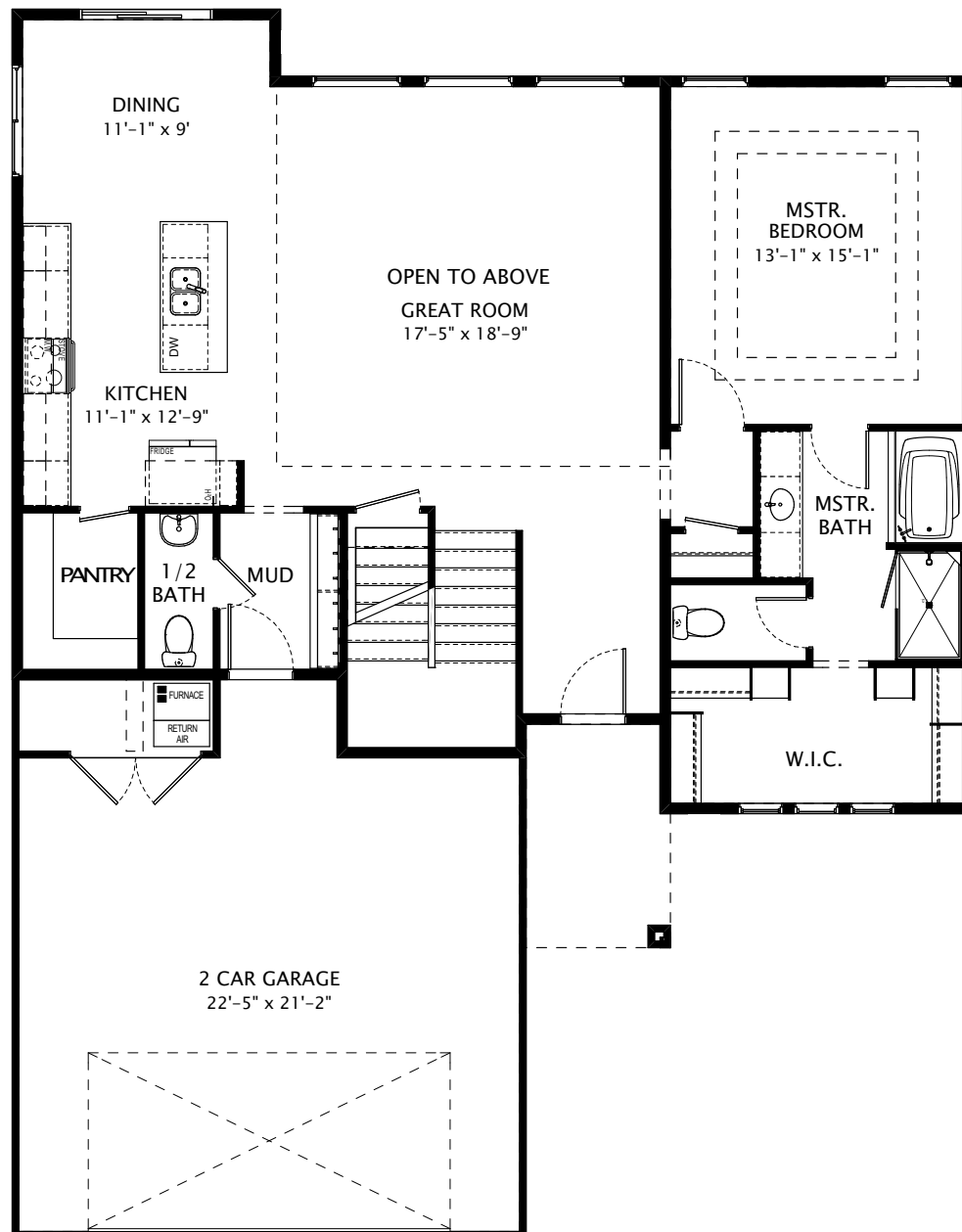
Main Floor
