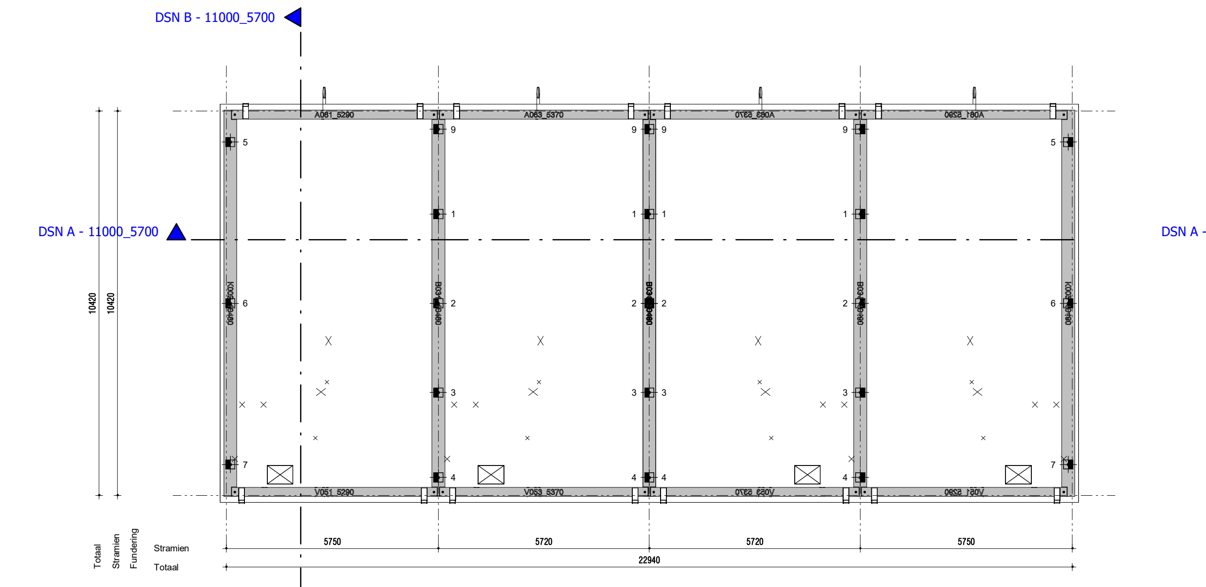
Fundering
