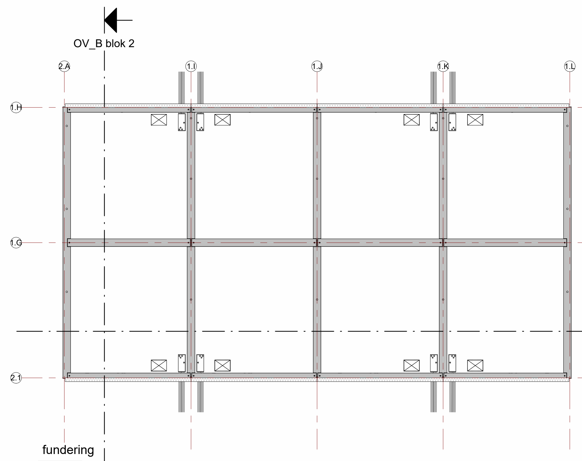
fundering
