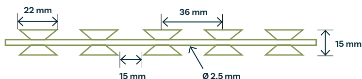
BTO 22 dimensions
