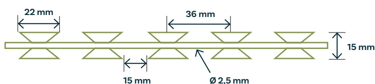
BTO 22 dimensions
