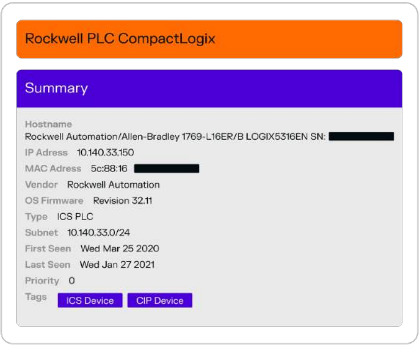
Figure 01: Device summary as identified by Darktrace / HYBRID NETWORK
