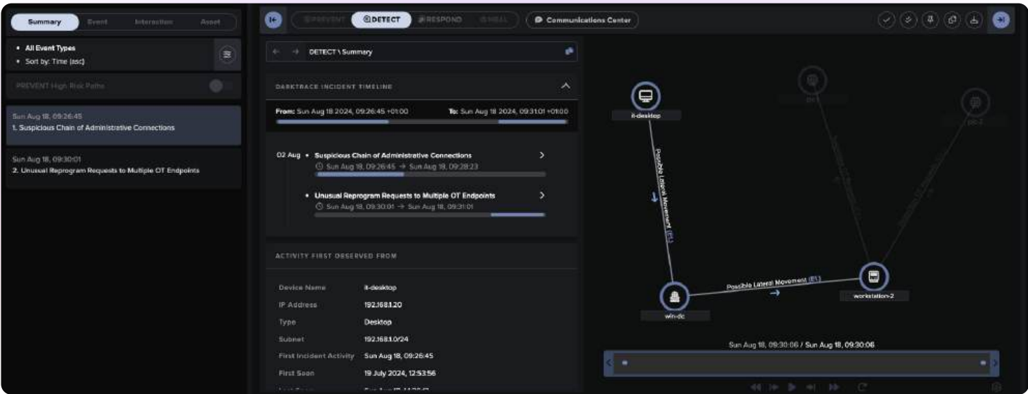
Figure 03: Cyber AI Analyst incident reporting on a potential insider threat with complete investigation process explained. A statistically unusual reprogram command was observed source device engineering workstation and destination PLC
