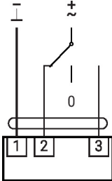
AC/DC 24 V, 3-point
