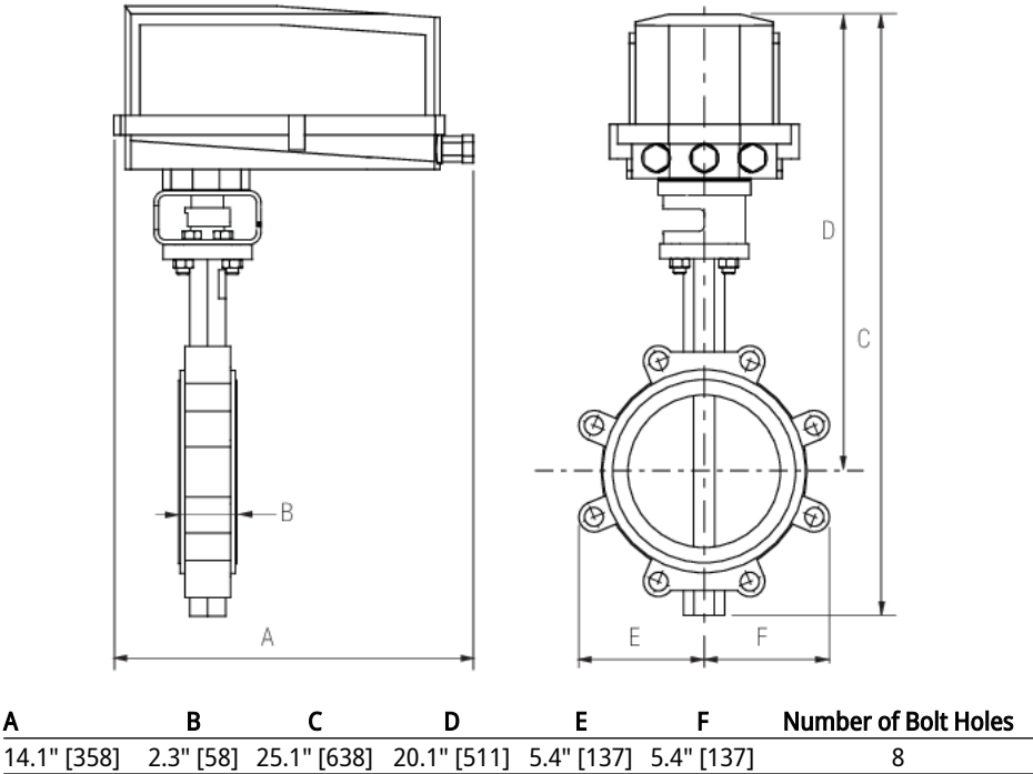
Valve with DR N4/DK N4 Actuator
