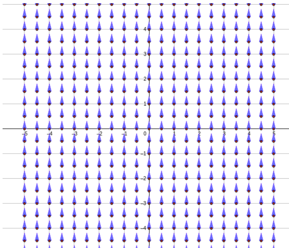
Figura 4: (r', \theta') = (0, 1)
