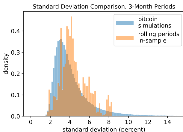
Fig. 6. A comparison of the standard deviation of Bitcoin from the model simulations, and the same standard deviation from rolling 3-month periods in the data.
