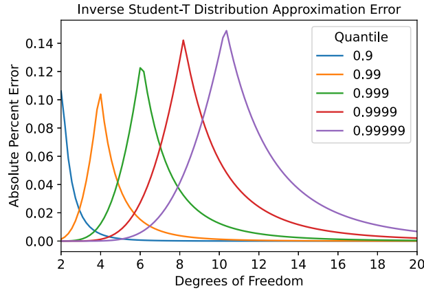
Fig. 19. The percent error in the combined inverse Student-t distribution approximation, switching between the Cornish-Fisher and tail series based on the fitted logistic function.
