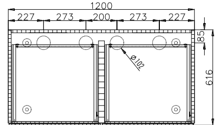
R 70/R 71 Container
