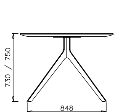
R 07 Side view
